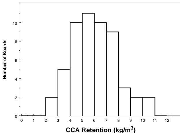
Figure 6 Range of CCA retentions measured in 2 by 6 Southern Pine lumber treated to target retention of 6.4 kg/m 3 .
