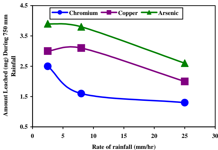
Figure 3 Effect of rate of rainfall on leaching of chromium, copper, and arsenic from CCA treated decking.
