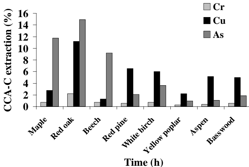
Figure 1 Relative leaching of CCA components from different species (AWPA E11 leaching test) [8].
