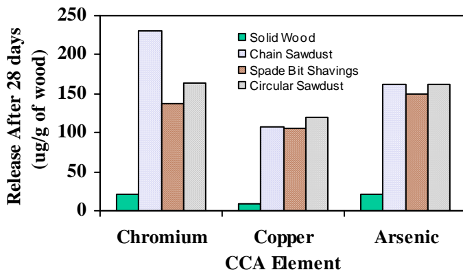
Figure 5 Comparison of amount of preservative released from solid wood or construction debris.
