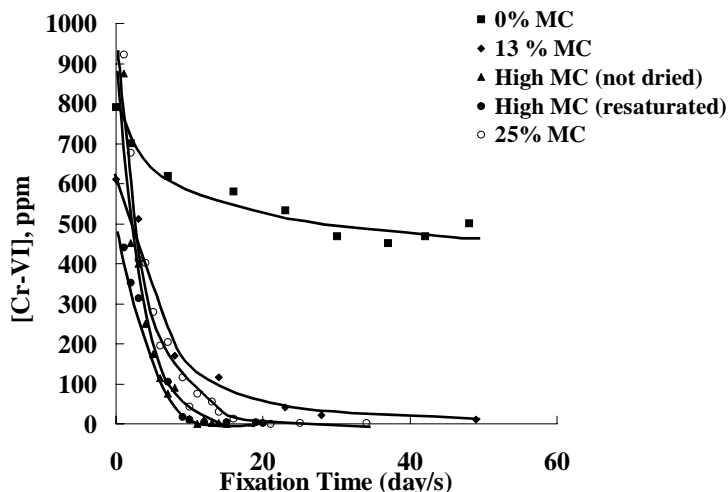
Figure 2 Effect of wood moisture content on chromium fixation.
