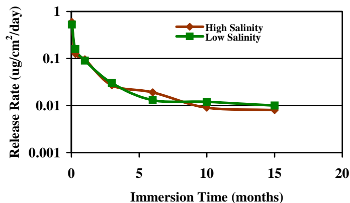
Figure 4 Change in rate of arsenic release from CCA treated 2 by 4 specimens immersed in seawater.
